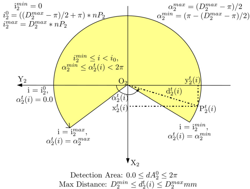
Fig. 7. Field of View of the rear Laser Scanner 2.
