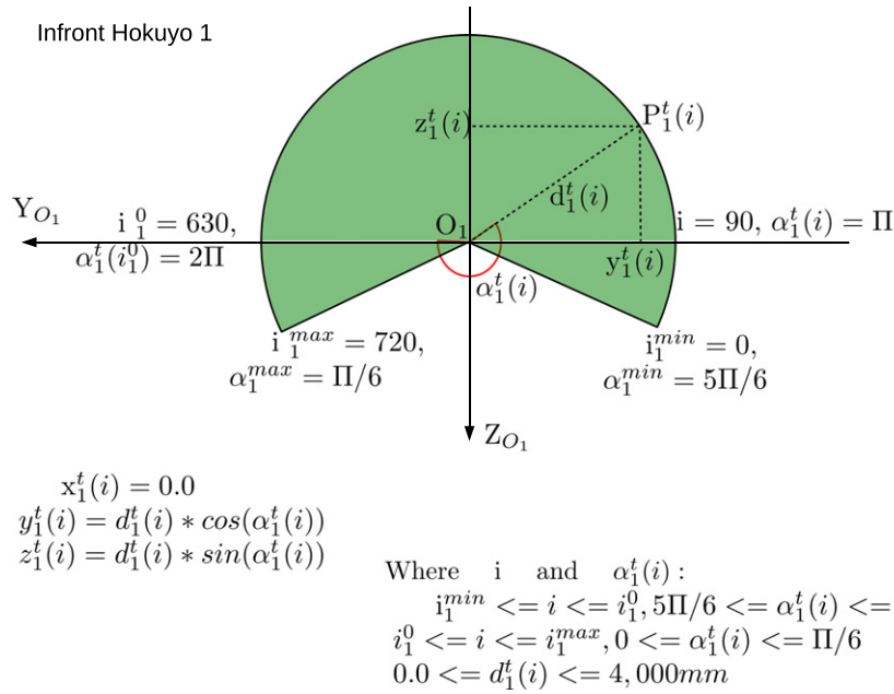
Fig. 10. Converting scanning points into 3D body frame of Hokuyo 1.
