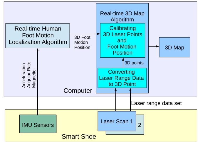
Fig. 2. The Smart Shoe's Components.
