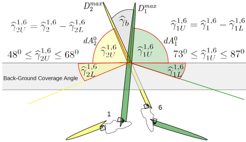
Fig. 5. The Smart Shoe scanning field estimation.
