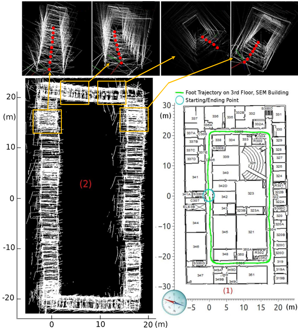
Fig. 12. The obtained 3D map of the 3rd floor hallway associated with foot’s trajectory in the SEM building by using our Smart Shoe. (1) Trajectory of the foot during walking in a closed loop with an indication of starting and ending positions. (2) A 3D map of the hallway during walking with some zoom-in areas.
