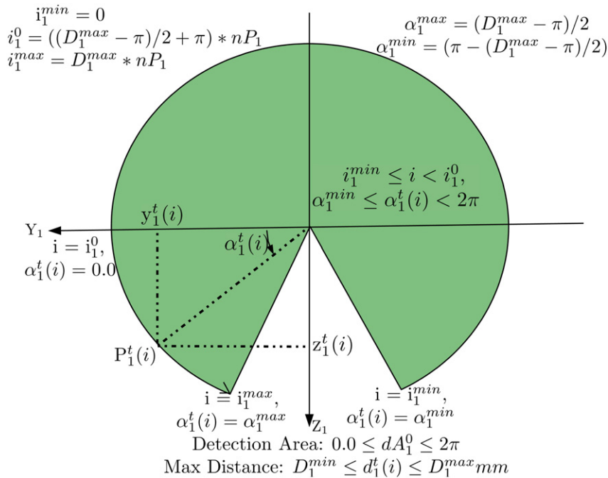
Fig. 6. Field of View of the front Laser Scanner 1.
