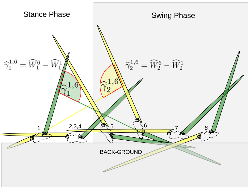
Fig. 4. The Smart Shoe scanning field by Gait Phase.
