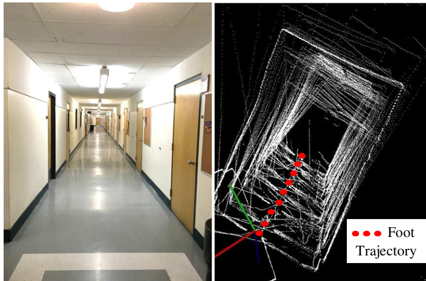
Fig. 13. Visual image of the hallway versus the 3D map.
