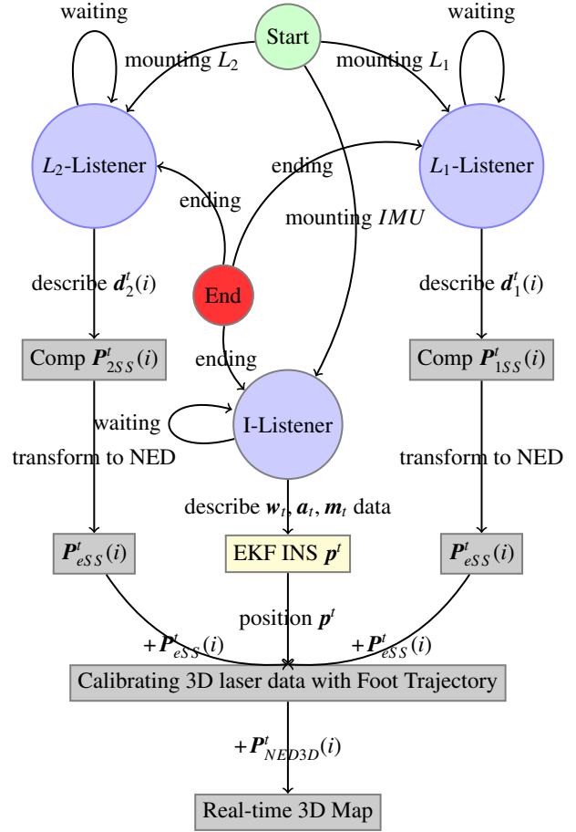
Fig. 8. A Real-time 3D mapping algorithm.
