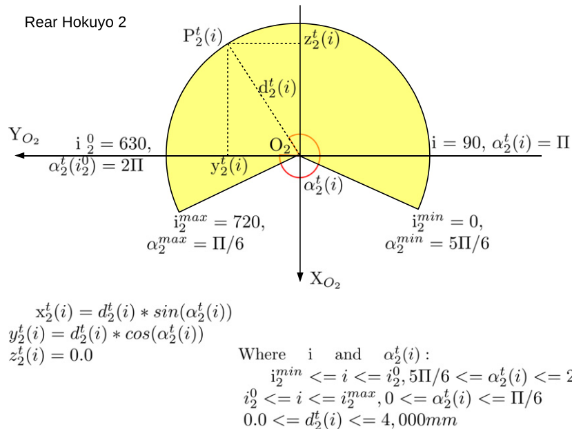
Fig. 11. Converting scanning points into 3D body frame of Hokuyo 2.
