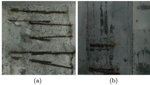
Fig. 1. Concrete spalling: (a) Large or very severe. (b) Small or less severe.
