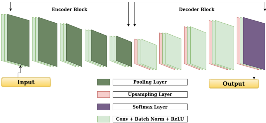
Fig. 3. Architecture for SegNet with encoder and decoder [14]
