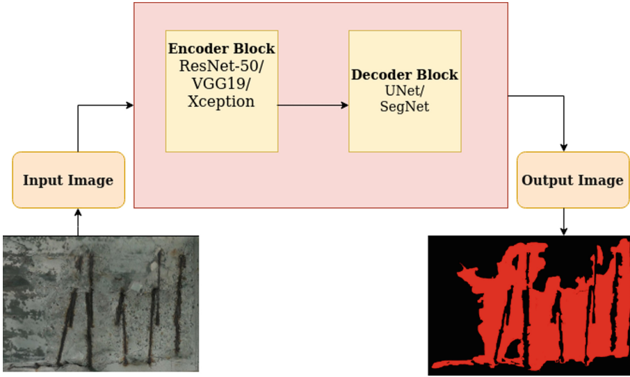
Fig. 4. Proposed encoder-decoder based deep architecture
