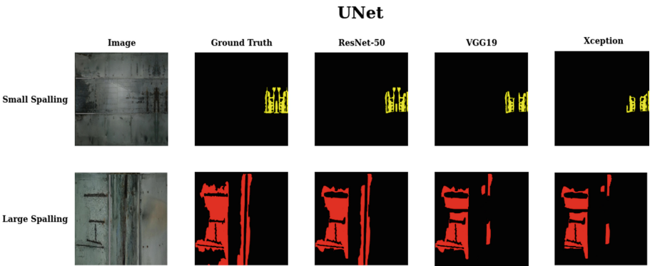
Fig. 5. Results shown for UNet framework with different encoder-decoder networks
