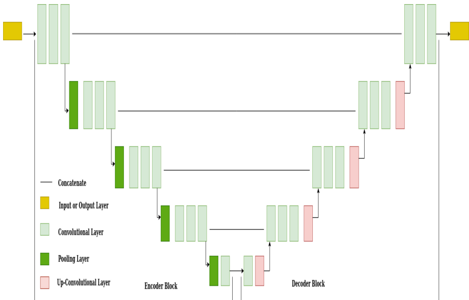
Fig. 2. Architecture for UNet with encoder and decoder [16]
